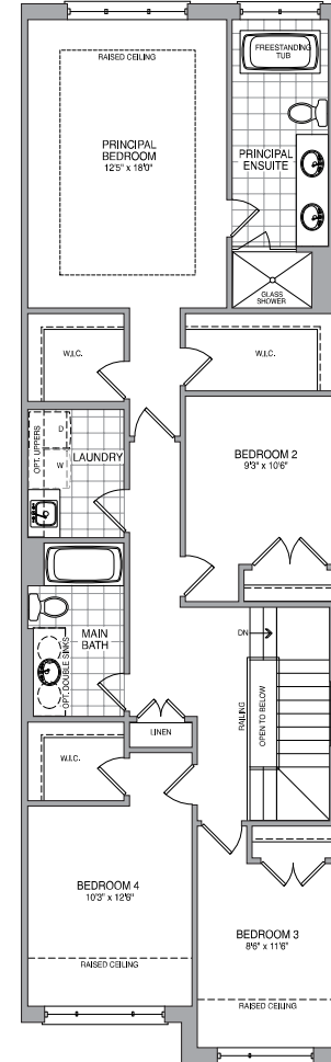
Upper Floor ELEVATION C
